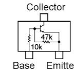
DTC114YUA (64) (Q6506)
