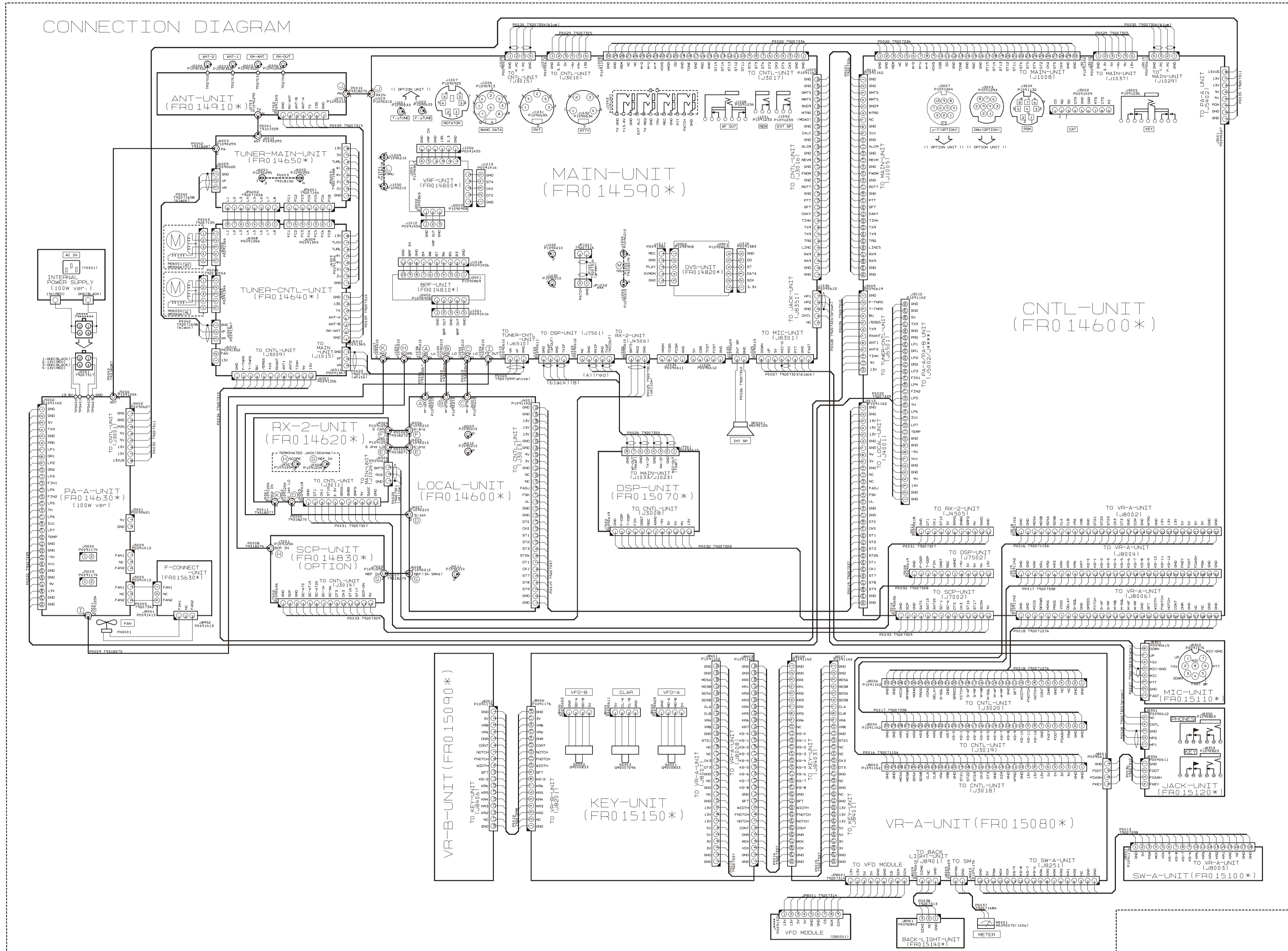
CONNECTION DIAGRAM-1
